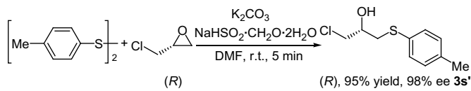
Scheme 2. The thiolysis of chiral epoxides.
