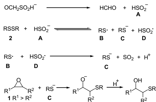
Scheme 3. A possible mechanism.
